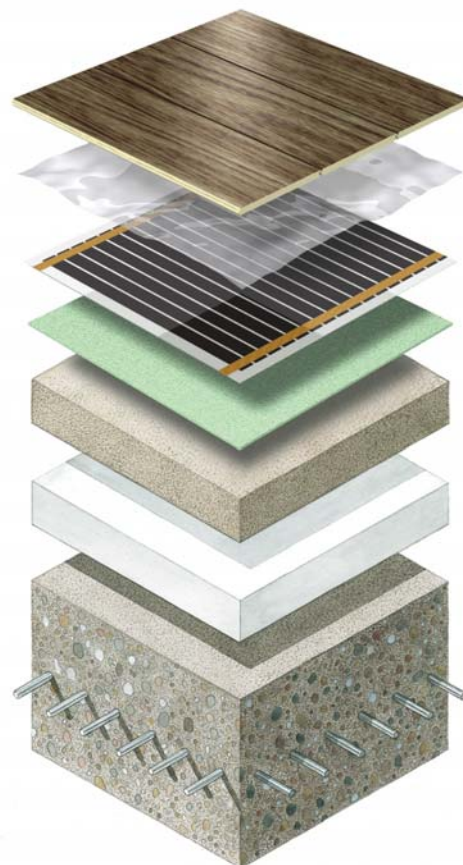
Use of Thermonet Foil in a solid floor application.
